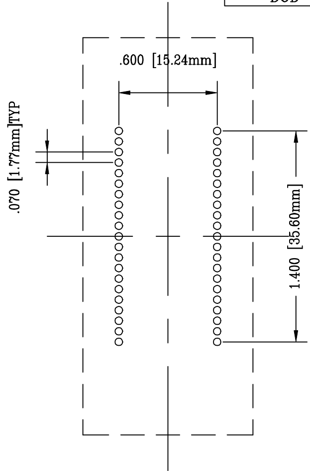
RECOMMENDED PCB LAYOUT AS SEEN FROM TOP OF SOCKET
