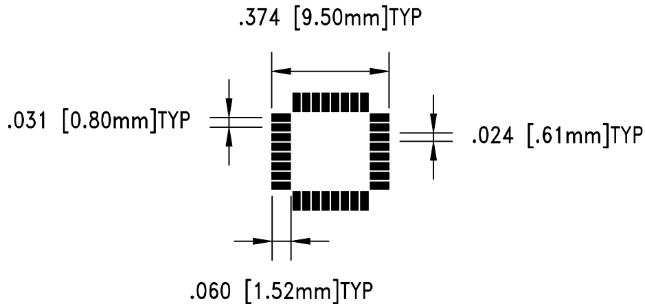
RECOMMENDED FOOTPRINT SCALE 2:1
